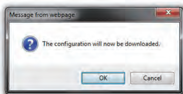
Figure 46 - Confirmation Prompt
